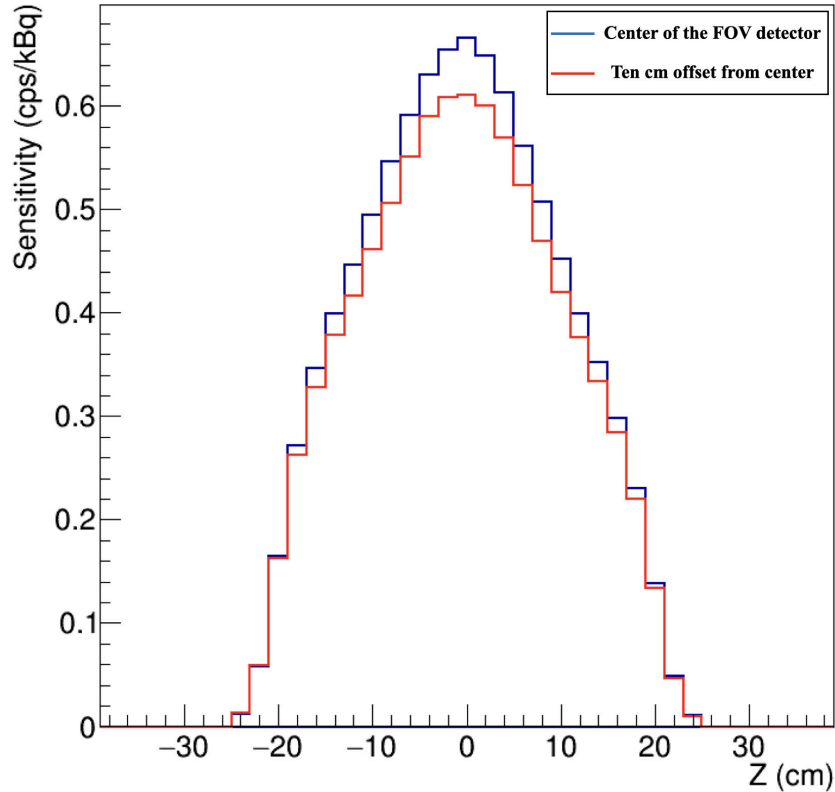
Rysunek 8.6: Axial sensitivity profile for the smallest sleeve in both positions.
