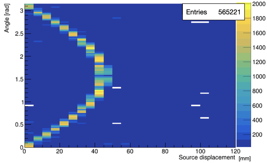
Rysunek 6.5: Illustrates sinogram was obtained as a sum of all aligned sinograms for whole scanner.
