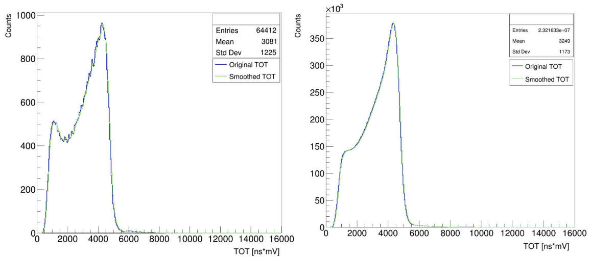
Rysunek 7.26: (Left): The histogram of TOT values for the scintillator ID =208 after correction. (Right): The sum histogram of TOT values is derived from the y-projection of the left plot, encompassing all scintillators after correction.
