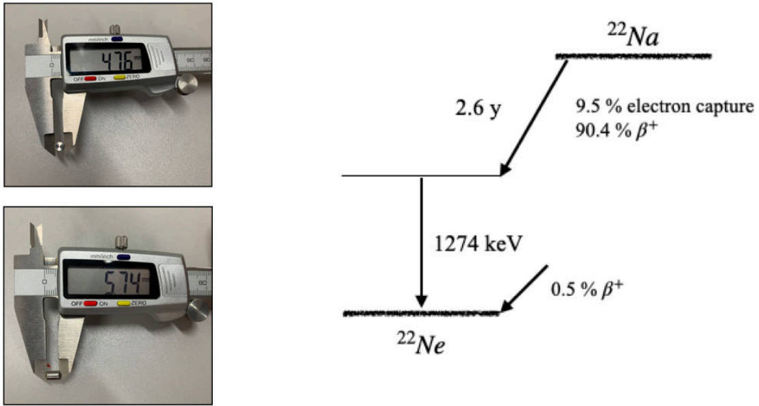
Rysunek 7.2: (Left): ^{22}\text{Na} Point source inside the stainless steel cylinder with outside diameter of 4.76 mm and 5.74 mm length, (Right) : Schematic of ^{22}\text{Na} decays. Figure adapted from [107].
