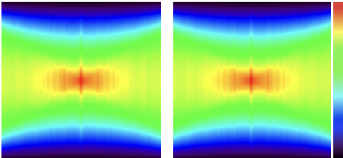
Rysunek 6.10: Transverse plane (-25 cm , 25 cm) representation extracted from the sensitivity map of the Modular J-PET, generated using QETIR software.
