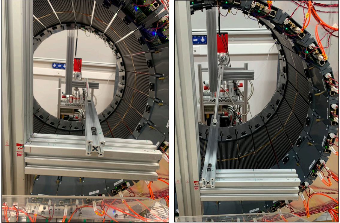
Rysunek 7.9: (Left): Depicts the arrangement of the 5 sleeves of the sensitivity phantom inside the Modular J-PET, positioned at the center of the detector. (Right): Displays the arrangement of the 5 sleeves of the sensitivity phantom inside the Modular J-PET, positioned at a 10 cm offset from the center.
