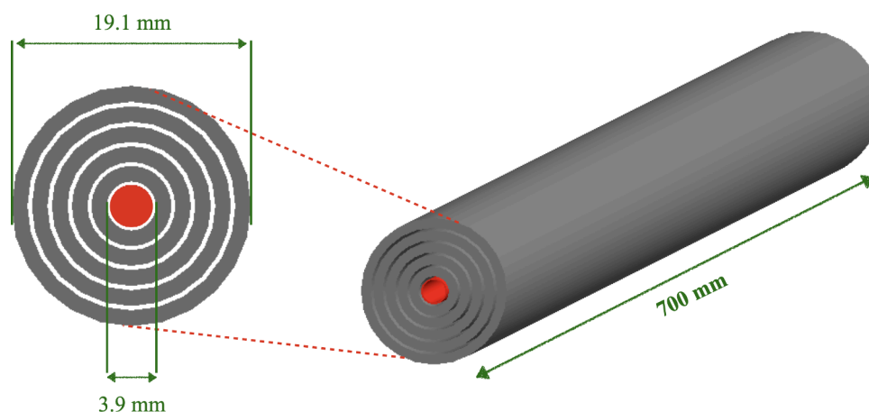
Rysunek 5.4: (Right): GATE visualization of sensitivity Phantom with five sleeve tubes displayed with gray and one polyethylene tube with length of 70 cm displayed with red. (Left) illustration of sensitivity phantom cross section, red point represented the line source inside the phantom. The figure isn't to scale.
