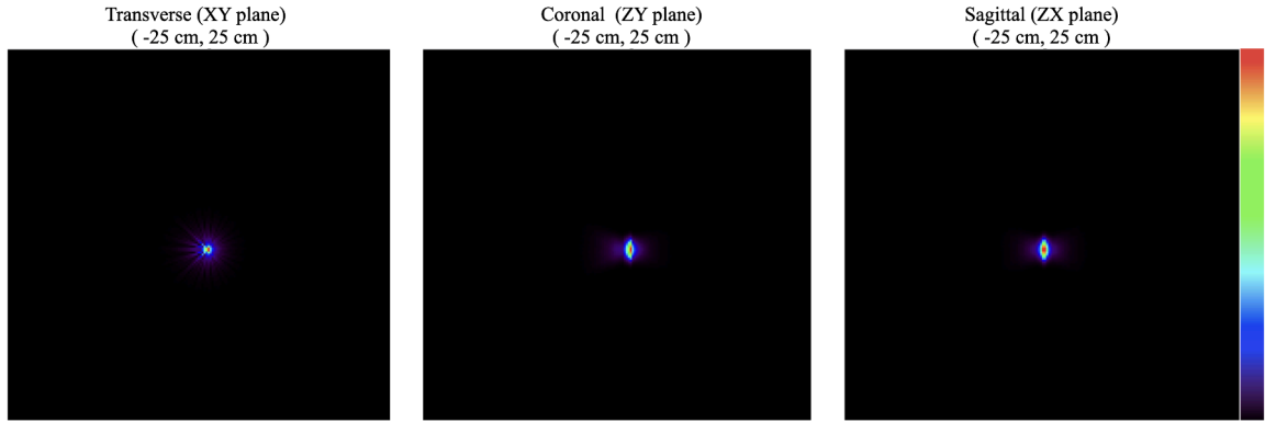
Rysunek 6.13: The outcomes of image reconstruction were generated using Non-TOF List Mode data for the source positioned at (1,0,0). The displayed images were obtained from the first iteration and showcase the reconstructed image in three directions.
