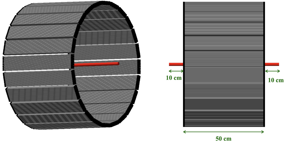
Rysunek 6.1: (Left): GATE visualization of the Modular J-PET with sensitivity phantom located in the center of the FOV. (Right) illustration of side view of the simulated sensitivity measurement, presenting place of source and phantom. The figure isn't to scale.
