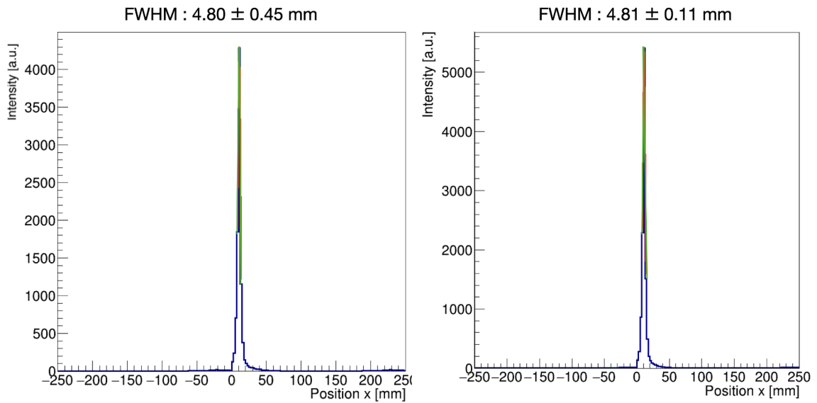
Rysunek 6.14: FWHM and its uncertainty estimation for distribution along x -axis performed at position (1,0,0), (left ) for TOF reconstructed image, and (right) Non-TOF reconstructed image.
