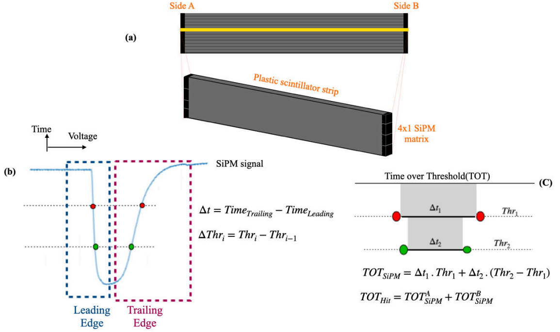
Rysunek 3.7: Reconstruction of SiPM signal in the Modular J-PET detector: (a) a single Module with a zoom on a single scintillator strip is represented, where scintillation light produced in a single scintillator strip is read out by a 4x1 matrix of SiPM-s on each side of the strip. (b) The collected light by the photomultiplier is converted into an electrical signal, which is characterized by a voltage dependence over time, denoted as V(t) . The dots represent the crossing of signals with the voltage threshold with nominal values: -30 and -70 mV. Front-end electronics measure times of each signal crossing two predefined voltage thresholds at its leading and trailing edge. (c) The size of the SiPM signal, which is related to the amount of scintillation light, is estimated using a rectangular approximation based on threshold levels above the signal baseline and the times-over-threshold (TOT) t_1 and t_2 , which are the differences between the trailing and leading edge times on each of the two voltage thresholds. Finally, the sum of the TOT values measured at both sides (side A and B) of the scintillator strip is used, as TOT characterizes the energy loss associated with the hit in the event.
