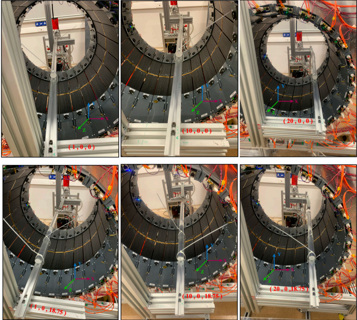
Rysunek 7.7: Six different positions inside the Modular J-PET scanner of sodium point like source placed in the plexi rod.
