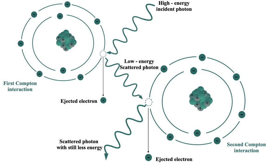
Rysunek 2.1: The Compton scattering process in which a gamma ray transfers only a portion of its energy to an electron in a shell, resulting in its own scattering with reduced energy. Figure adapted from [39].
