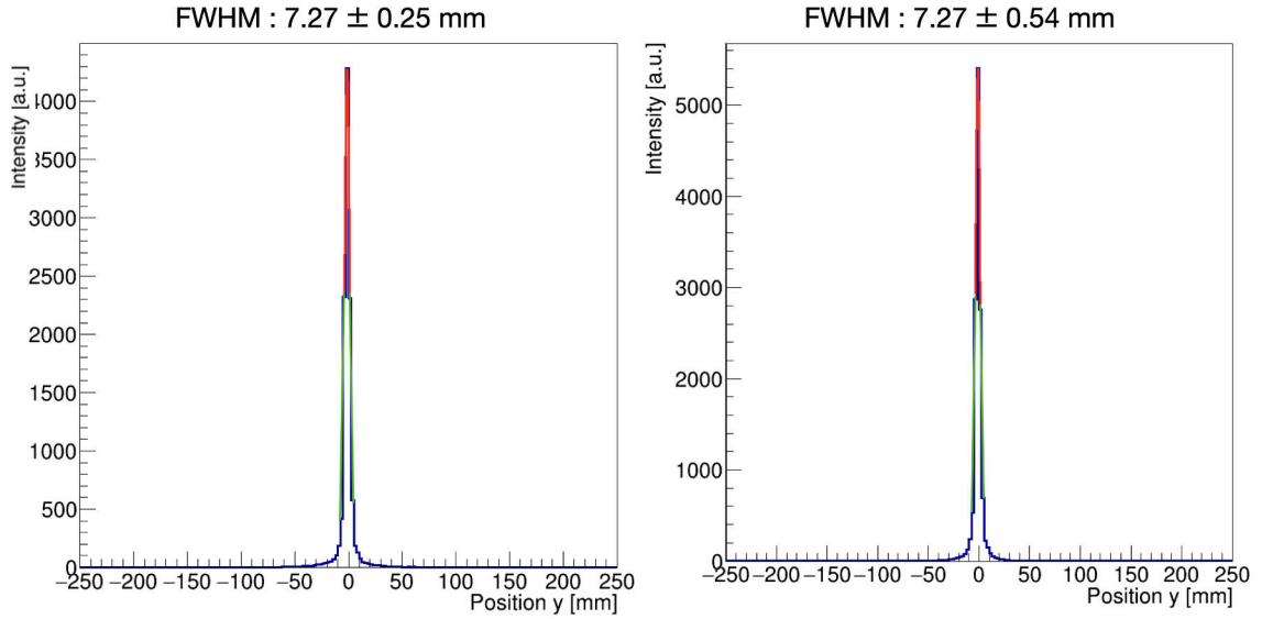
Rysunek 6.15: FWHM and its uncertainty estimation for distribution along y -axis performed at position (1,0,0), (left ) for TOF reconstructed image, and (right) Non-TOF reconstructed image.
