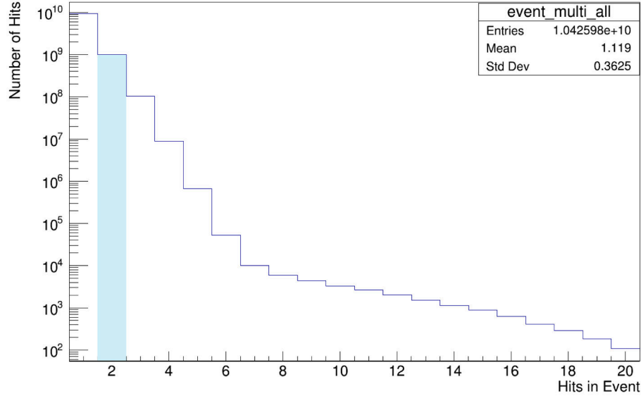
Rysunek 7.14: The distribution of the multiplicity of the hits in event in 4 ns coincidence time window in logarithmic scale. In this case, only the events with two hits were taken into account.
