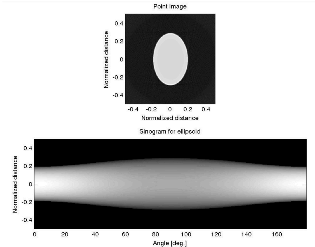
Rysunek 2.12: Example of sinogram for point in the center of scanner. Figure adapted from [72].
