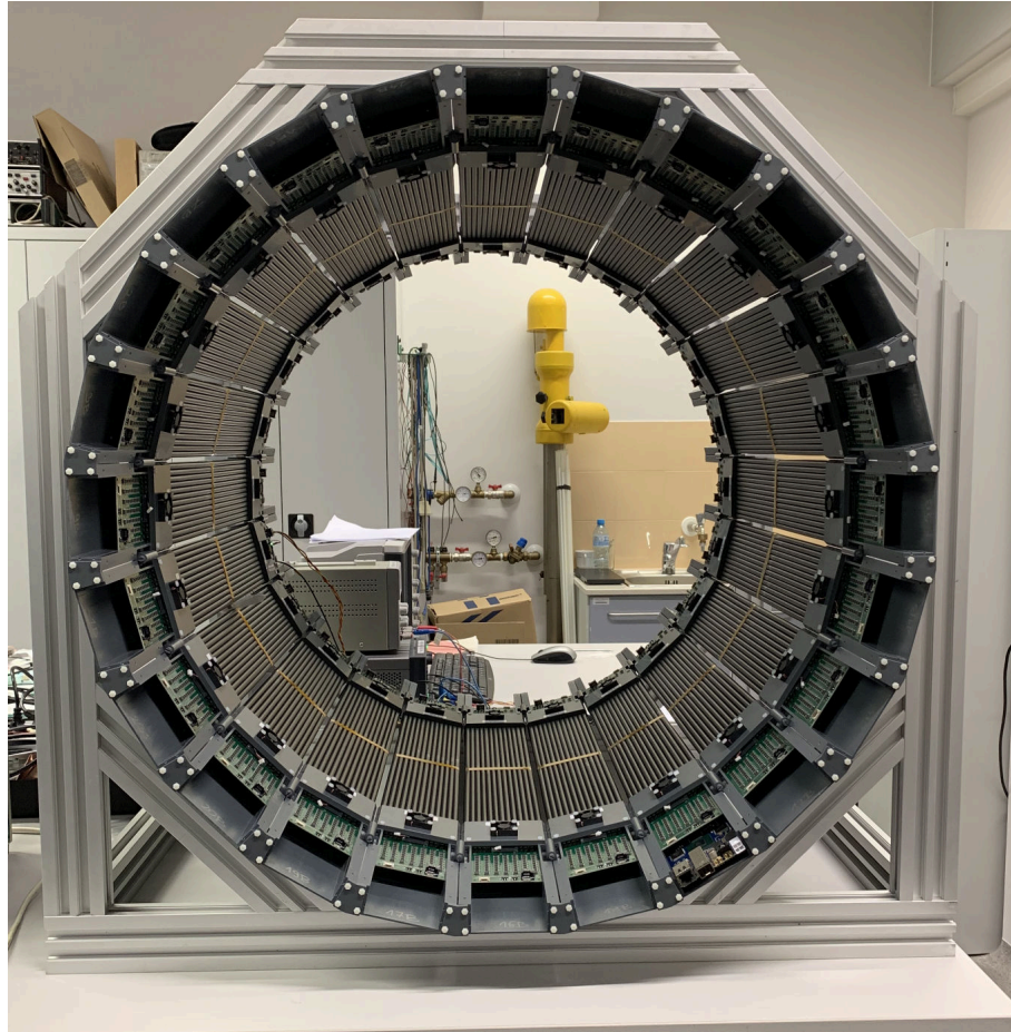
Rysunek 3.4: Illustration of the Modular J-PET.
