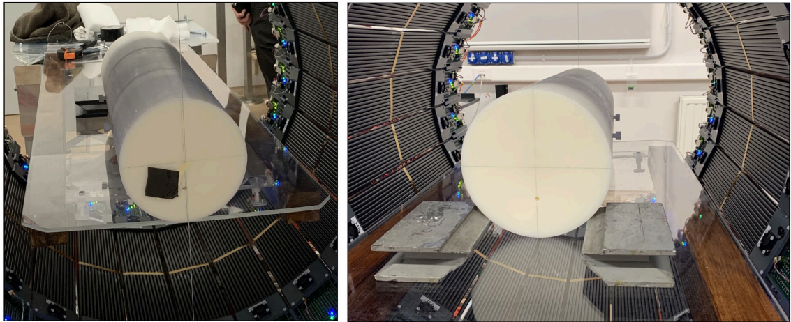
Rysunek 7.11: (Left): Visible in this image is a taut thread running along the y-axis. The line on the phantom's edge conceals the positions of these threads. Additionally, the remainder of the line source is depicted as extending beyond the phantom's boundaries. (Right): This image showcases the phantom supported on both sides.
