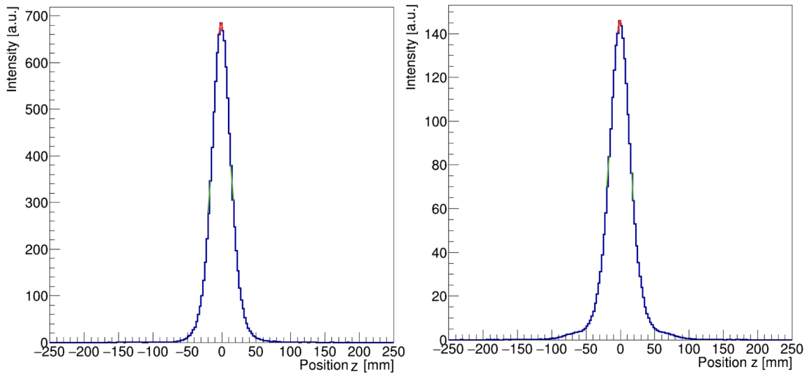
Rysunek 8.24: FWHM and its uncertainty estimation for distribution along z -axis performed at position (1,0,0), (left ) for TOF reconstructed image, it is equal to 29.51 \pm 0.52 \text{ mm} , and (right) Non-TOF reconstructed image, it is equal to 34.43 \pm 0.10 \text{ mm} .
