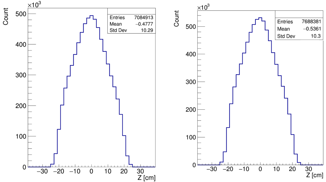
Rysunek 8.3: The Z projection has been generated using information regarding the annihilation position for a source positioned at the center of the detector's AFOV. On the left, the projection represents data for a single sleeve, while on the right, it illustrates the information gathered from five sleeves.
