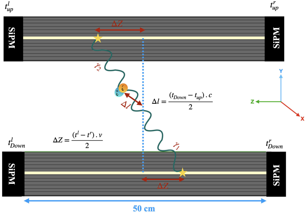
Rysunek 3.1: Two detection module setup with scintillators and SiPMs arrangements, principle of detection and reconstruction of annihilation positions in the J-PET plastic scintillator based technology where the axially arranged scintillator (gray) is readout by two photomultiplier of both ends (black).
