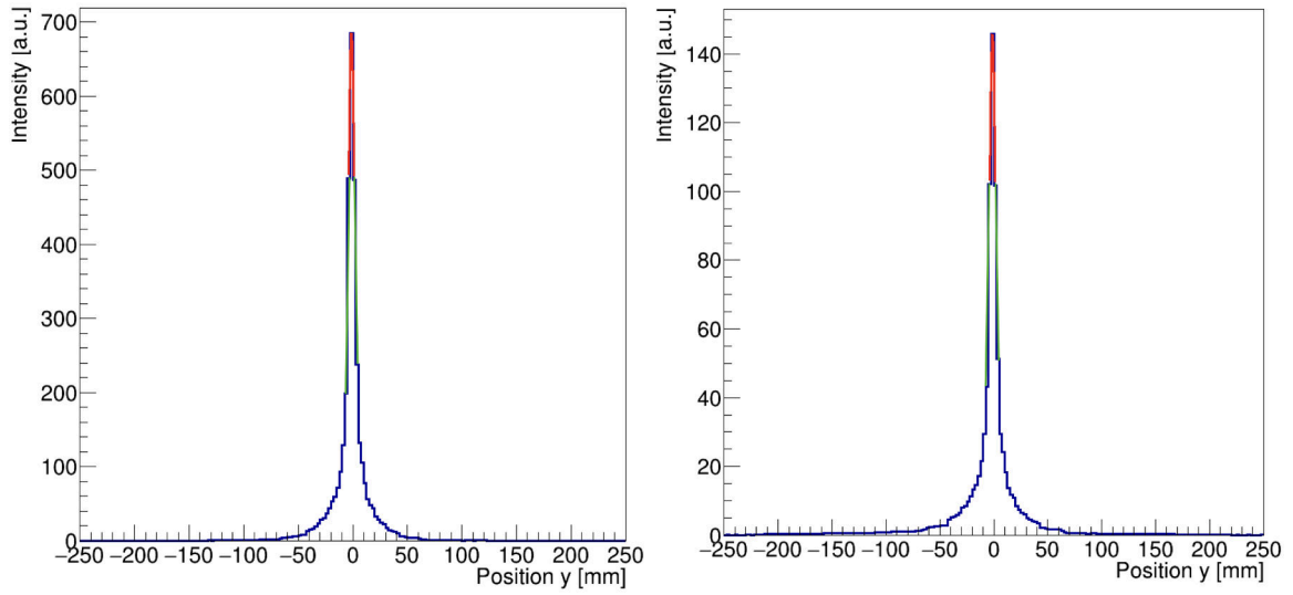
Rysunek 8.23: FWHM and its uncertainty estimation for distribution along y -axis performed at position (1,0,0), (left ) for TOF reconstructed image, it is equal to 7.38 \pm 0.54 \text{ mm} , and (right) Non-TOF reconstructed image, it is equal to 7.38 \pm 0.11 \text{ mm} .
