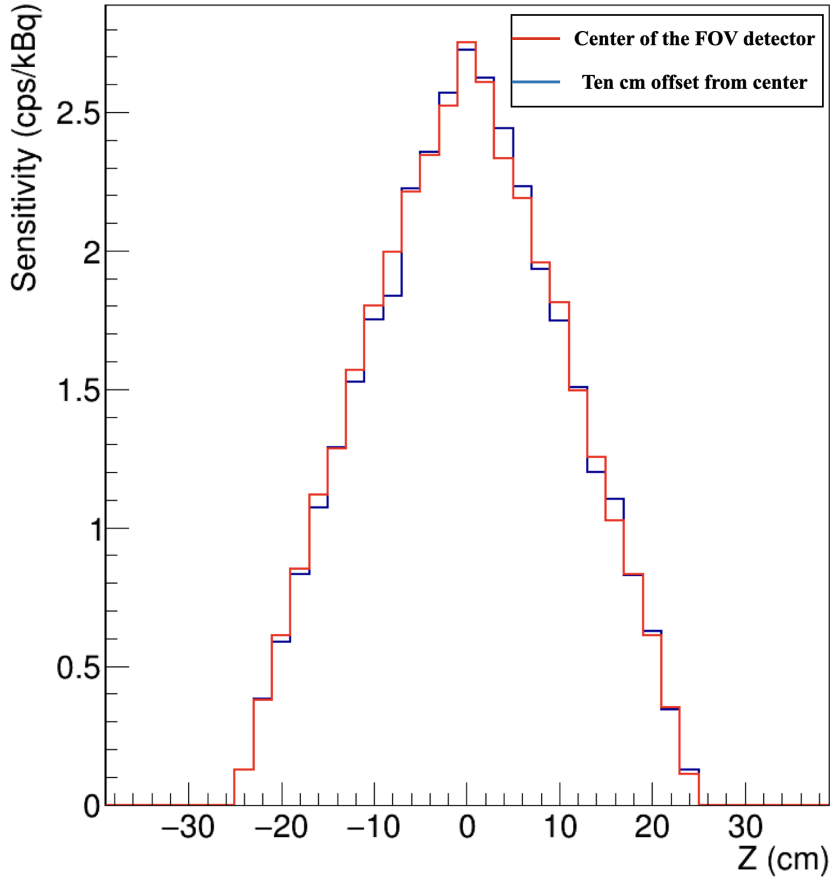
Rysunek 6.3: Axial sensitivity profile for the smallest sleeve in both positions. The peak sensitivity value is equal to 2.8 cps/kBq in the center of the scanner FOV and 2.75 cps/kBq in 10 cm offset from the tomograph center.
