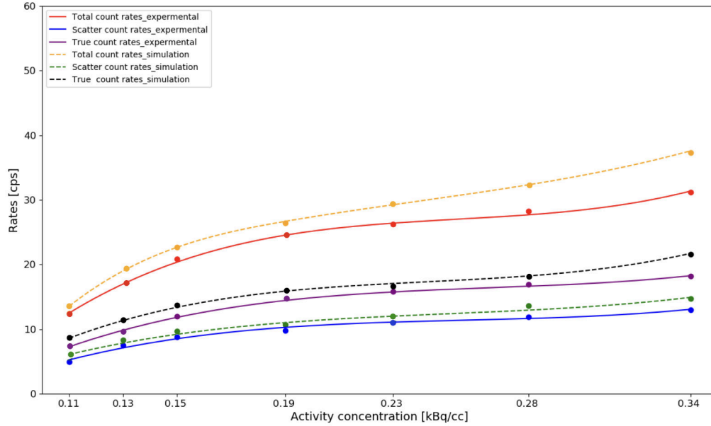
Rysunek 10.2: Comparison Plots: Simulated and Experimentally Measured Total, True, and Scatter Coincidence Count Rates as function of average activity concentration (kBq/cc) for the 700 mm Long Phantom in the Modular J-PET Scanner.
