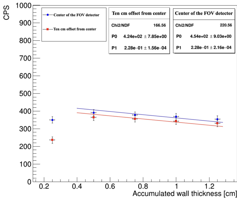
Rysunek 8.5: Illustrates how R_j (Counts Per Second) varies with the accumulated sleeve wall thickness. As depicted, there is a noticeable decrease in count rate as the wall thickness increases. These measurements were obtained at the center of the detector and at the ten cm offset from the center of the detector. The data is fitted with equation specified in Eq. 4.3.
