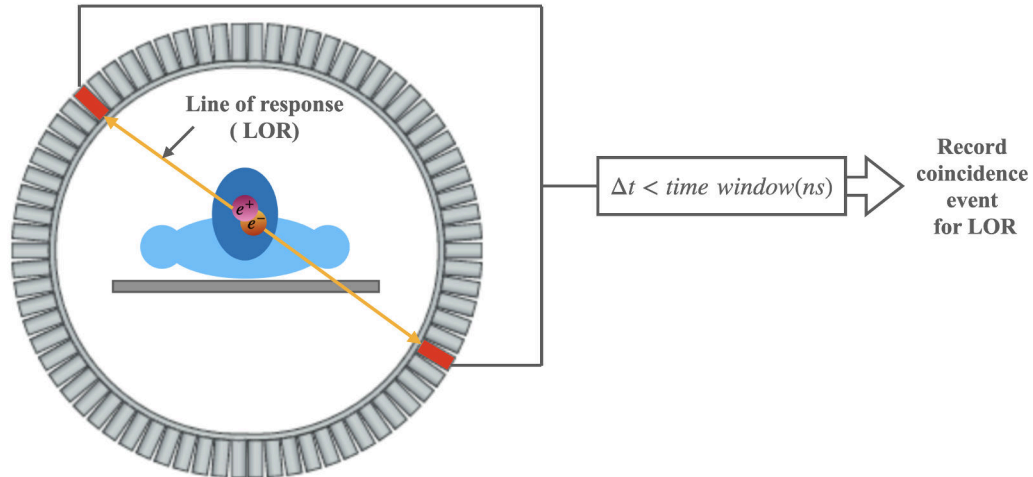
Rysunek 2.9: Coincidence event processing in PET data acquisition. Figure adapted from [70].
