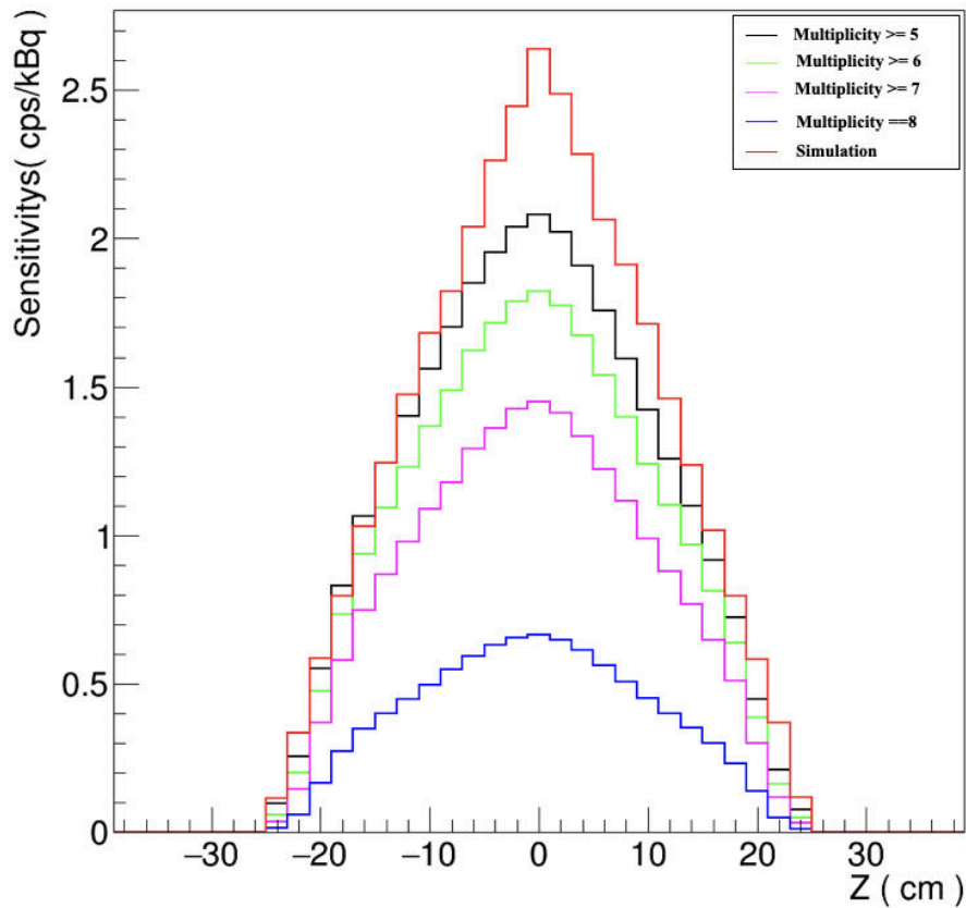
Rysunek 10.1: Axial sensitivity profile for the smallest sleeve in the center of the FOV detector for different multiplicity cuts. Red line presents the axial sensitivity profile for the center of the detector from simulation part.
