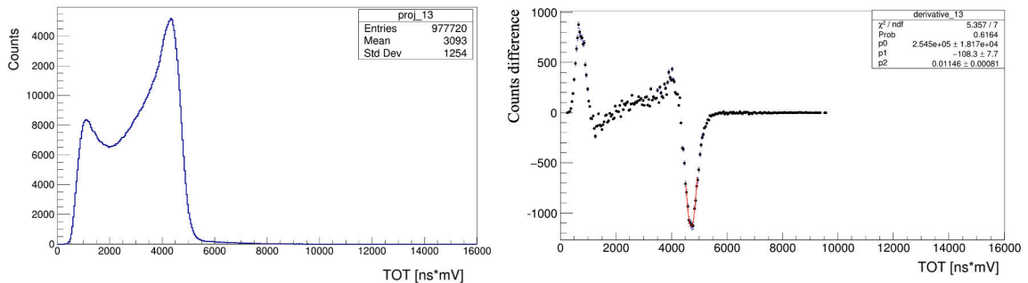
Rysunek 7.29: The TOT spectra depict individual results for each interaction points of gamma quanta along scintillators.
