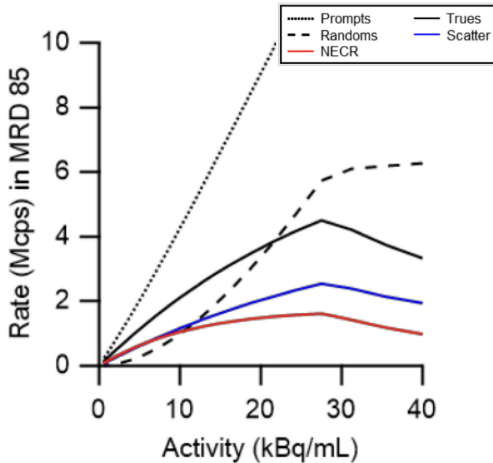
Rysunek 9.5: Graphs representing prompt, random, true, scatter, and NEC rates for MRD 85. Figure was adapted from [111].
