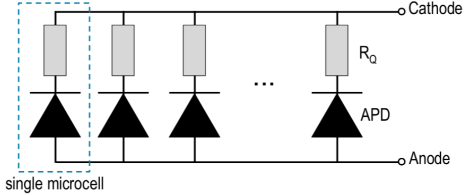
Rysunek 2.6: Schematic view of Silicon photomultiplier(SiPM) structure which All of the microcells are connected in parallel [59].
