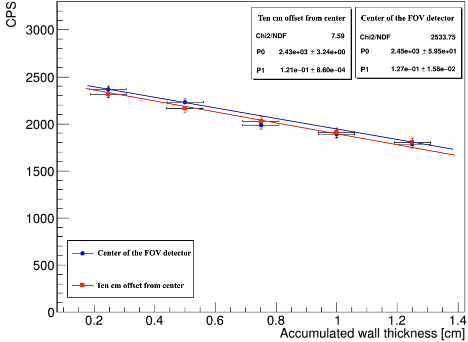
Rysunek 6.2: Illustrates how R_j (cps) varies with the accumulated sleeve wall thickness. As depicted, there is a noticeable decrease in count rate as the wall thickness increases. These measurements were obtained at the center of the detector and at the ten cm offset from the center of the detector, and the data is fitted to the equation specified in Eq. 4.3.
