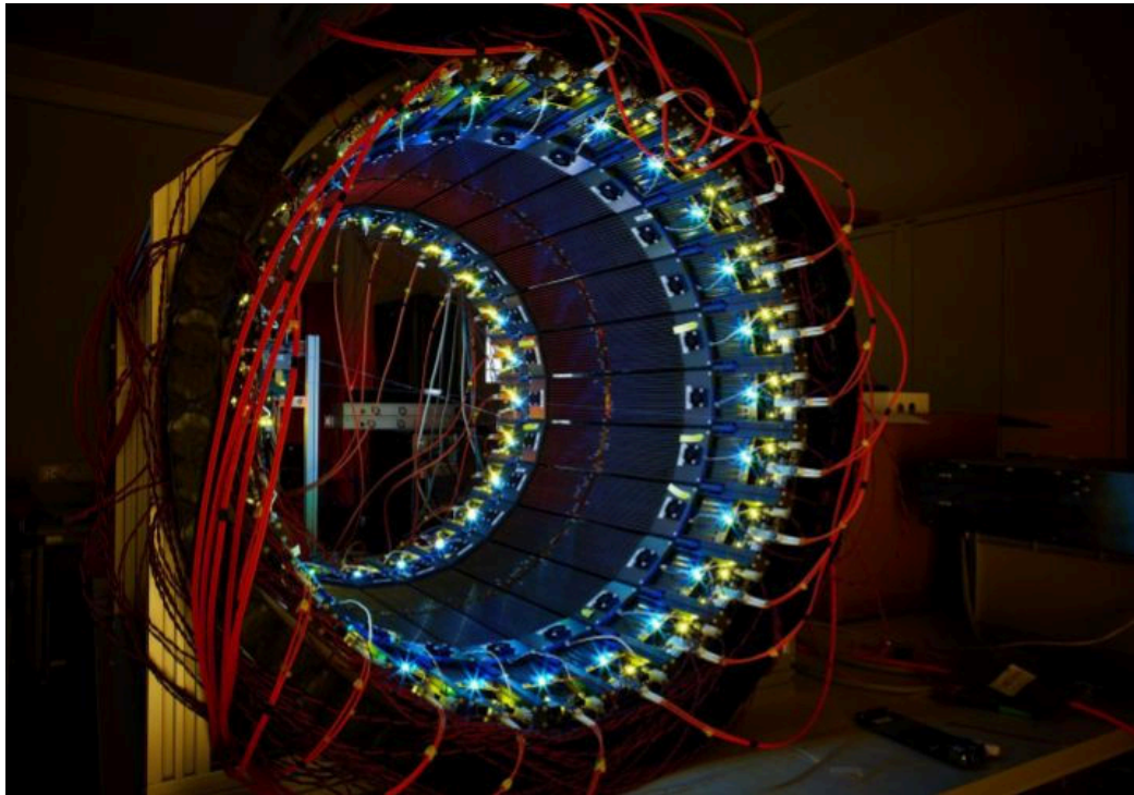
Rysunek 1.2: Modular J-PET detector, built out of 24 modules which each module is composed of 13 scintillator strips, read out by a silicon photomultiplier (SiPM) array from both sides.
