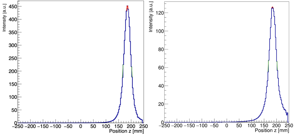
Rysunek 8.27: FWHM and its uncertainty estimation for distribution along z -axis performed at position (20,0,18.75) , (left) for TOF reconstructed image, it is equal to 34.43 \pm 0.28 mm, and (right) Non-TOF reconstructed image, it is equal to 35.00 \pm 0.09 mm.
