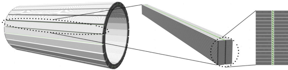
Rysunek 10.4: (Left) Visualization of the Total Body J-PET scanner with GATE software. (Middle) illustration of the panel composed of two modules. (Right) Transvers illustration of the detection panels and WLS (hashline pattern) in between. Figure is adapted from [104].
