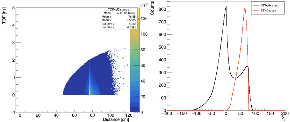
Rysunek 7.20: (Left): Two-dimensional histogram depicting the spatial separation as a function of Time of Flight (TOF) after adding \delta_{i,j} > 40 \text{ cm} , (Right): Illustrates comparison of the \delta_{i,j} = d_{i,j} - c \cdot \Delta t_{i,j} for all events and after adding \delta_{i,j} > 40 \text{ cm} . Only events with two primary photon interactions remaining after the selection are used to construct LOR-s for image reconstruction.
