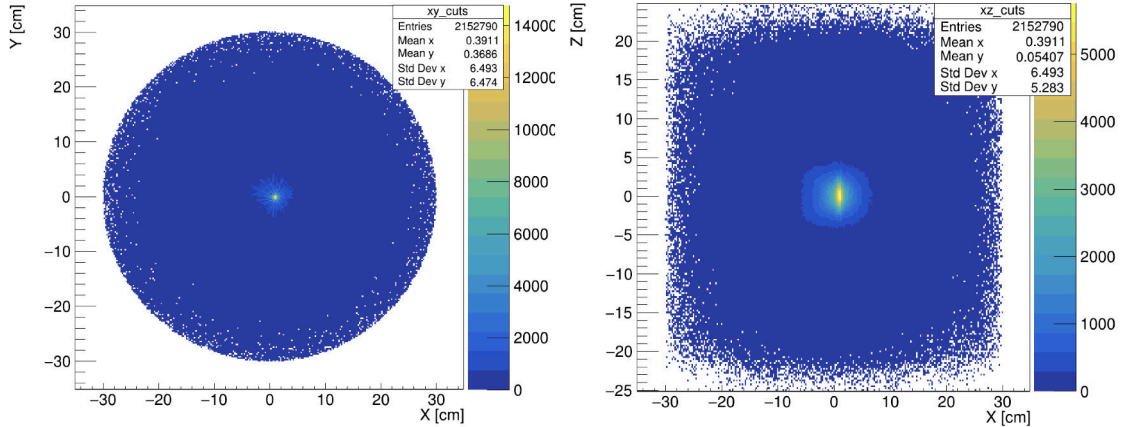
Rysunek 8.15: Histogram of annihilation points for position (1,0,0): (Left) XY projection of annihilation point and, (Right) XZ projection of annihilation points.
