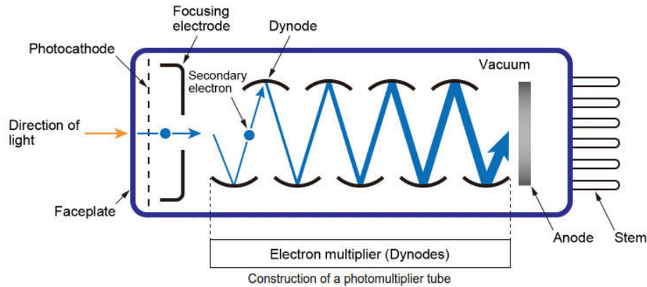
Rysunek 2.5: Schematic view of photomultiplier tube. Figure adapted from [55].
