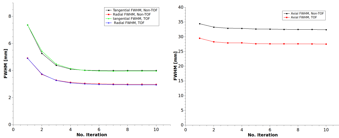
Rysunek 8.28: FWHM values as function of the iteration number for positions (1,0,0) in three direction. (left): Radial and tangential FWHM with TOF and Non-TOF image reconstruction methods, (right): Axial FWHM with TOF and Non-TOF image reconstruction methods. TOF image reconstruction methods is only improving axial PSF.
