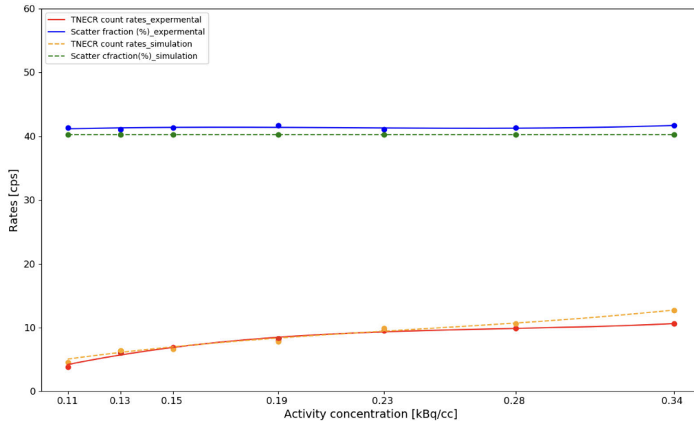
Rysunek 10.3: Comparison Plots: Simulated and Experimentally Measured NECR Count Rates and scatter fraction as function of average activity concentration (kBq/cc) for the 700 mm Long Phantom in the Modular J-PET Scanner.
