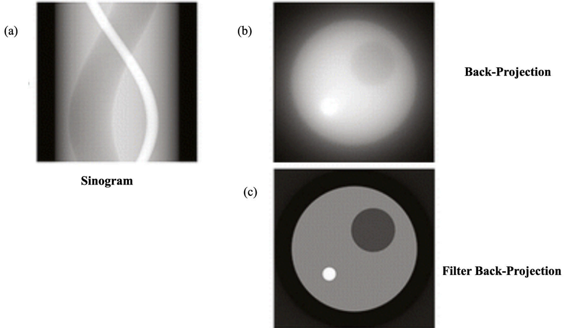
Rysunek 2.14: Comparison of the FBP method and BP method in PET image reconstruction. (a) Sinogram stored from data acquisition, (b) simple back projection algorithm method, (c) filtered back projection algorithm method. Figure adapted from [75].
