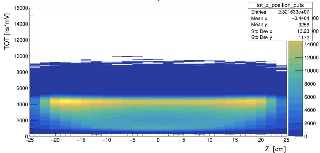
Rysunek 7.29: The TOT spectra depict individual results for each interaction points of gamma quanta along scintillators.
