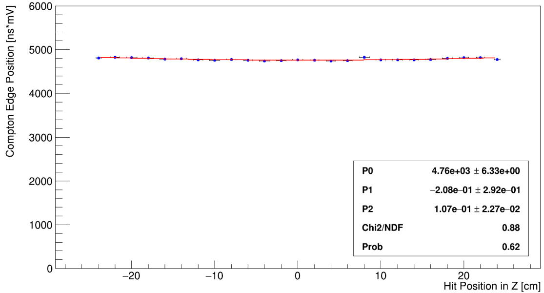
Rysunek 7.31: The values of Compton edges position have been determined for all the scintillators at 25 points of interaction along the z-axis. A quadratic function has been fitted.
