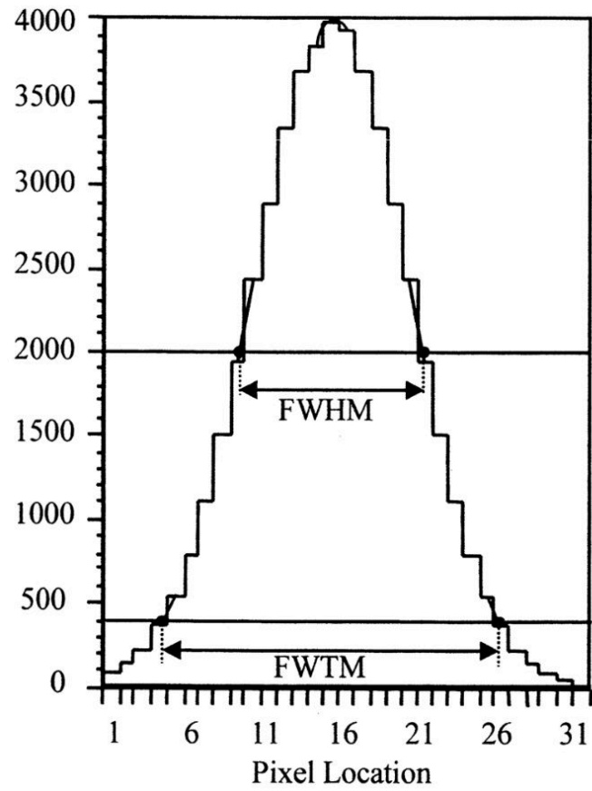
Rysunek 4.4: Illustrates the response function, with its FWHM and FWTM, is typically determined through graphical interpolation.
