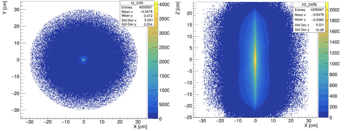
Rysunek 7.32: Control histogram of annihilation point after applying TOT rang to pre-selection criteria in 4 ns coincidence time window: (Left) XY position of annihilation point and, (Right) XZ position of annihilation point.
