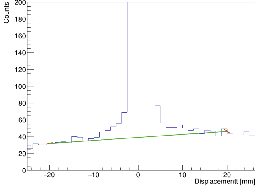
Rysunek 6.7: One-dimensional profile calculated as aligned to zero using maximum value and summed projections of sinogram, used to differentiate the true and the false (scattered and accidental) coincidences. Coincidences over the green line are treated as true coincidences, while those below as scattered and accidental ones.
