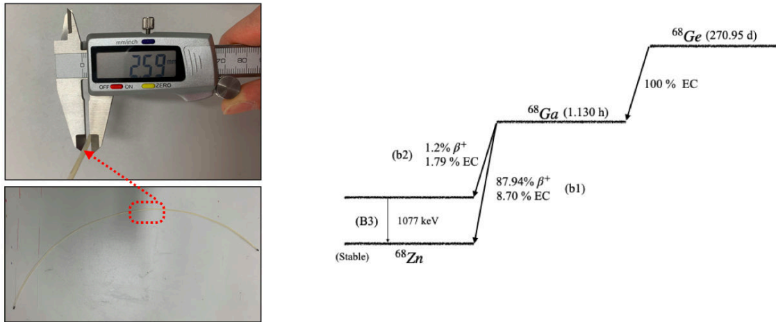
Rysunek 7.3: (Left): ^{68}\text{Ge} line source inside the polyethylene tube, 2.59 mm of the outside diameter of tube, (Right) schematic of ^{68}\text{Ge} decays. Figure adapted from [108].
