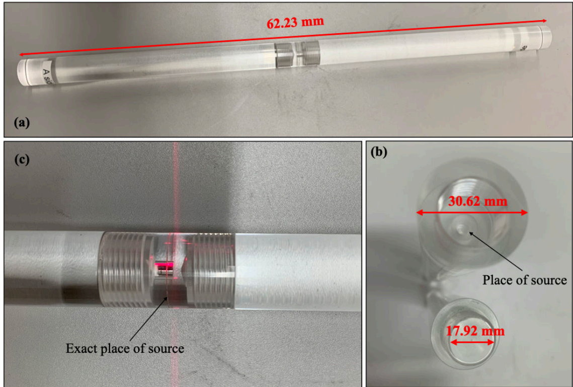
Rysunek 7.5: (a): The 62.23 mm length plexi rod for point source measurements in Modular J-PET detector spatial resolution experiment. (b) Cross-section of the middle of plexi rod with an outside diameter of 30.62 mm. Source is placed in the center of the plexi rod. (c): Place of the point like source in the plexi rod, the line in the plexi rod represented the exact place of source inside plexi rod.
