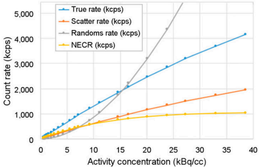
Rysunek 9.4: The results of the NEMA NU-2 count-rate performance, using a 70-cm line source placed within a 20-cm-diameter polyethylene scatter cylinder for the PennPET detector. Figure was adapted from [103].
