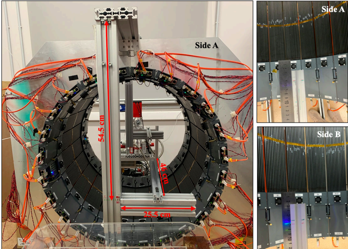
Rysunek 7.6: (left): Aluminum supports used to locate the plexi rod and sensitivity phantom inside the Modular J-PET scanner. (Right) Top view of the aluminum supports in both sides, showing that the aluminum supports are located outside of AFOV scanner at both sides.
