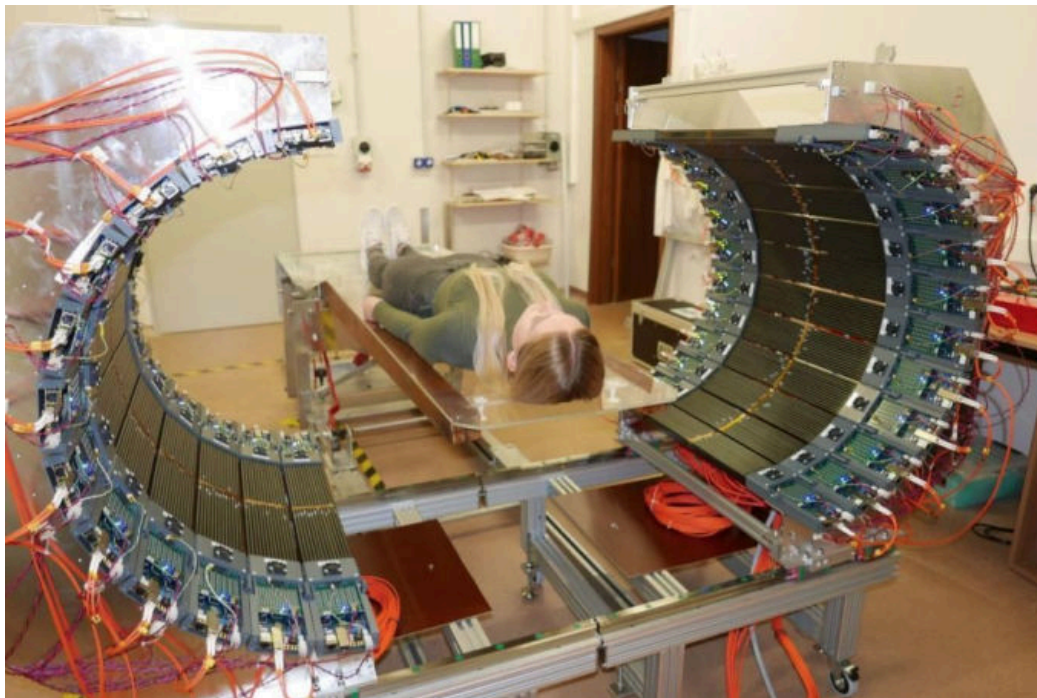
Rysunek 9.6: The Modular J-PET prototype, installed in the laboratory in the Jagellonian University, while it is being closed the system around a student already lying on the table.
