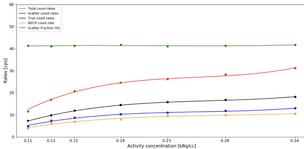
Rysunek 8.14: The count rates of various coincidence types, NECR, and scatter fraction (%) are typically plotted as functions of the average activity concentration (kBq/cc) for the Modular J-PET.
