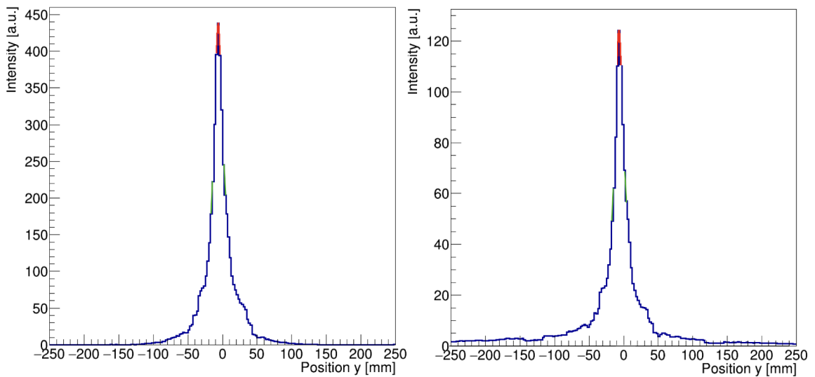
Rysunek 8.26: FWHM and its uncertainty estimation for distribution along y -axis performed at position (20,0,18.75), (left ) for TOF reconstructed image, it is equal to 17.21 \pm 0.32 \text{ mm} , and (right) Non-TOF reconstructed image, it is equal to 14.42 \pm 0.10 \text{ mm} .
