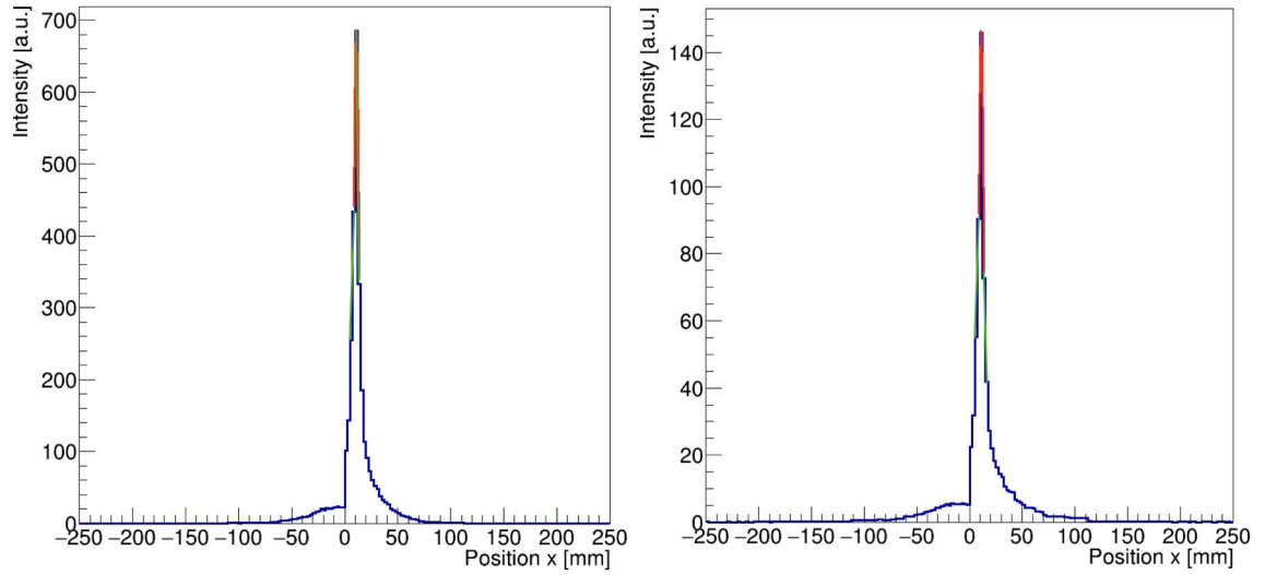
Rysunek 8.22: FWHM and its uncertainty estimation for distribution along x -axis performed at position (1,0,0), (left ) for TOF reconstructed image, it is equal to 4.92 \pm 0.55 \text{ mm} , and (right) Non-TOF reconstructed image, it is equal to 4.92 \pm 0.12 \text{ mm} .
