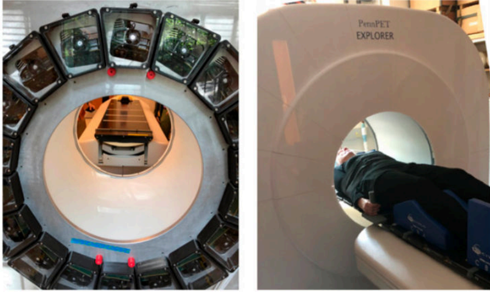
Rysunek 9.3: Prototype configuration of the PennPET Explorer, featuring three ring segments enclosed in a dry, cool environment. The rear view of the gantry exhibits modular detector and electronic bays, along with the couch featuring a flat pallet installed for human studies. Figure was adapted from [103].
