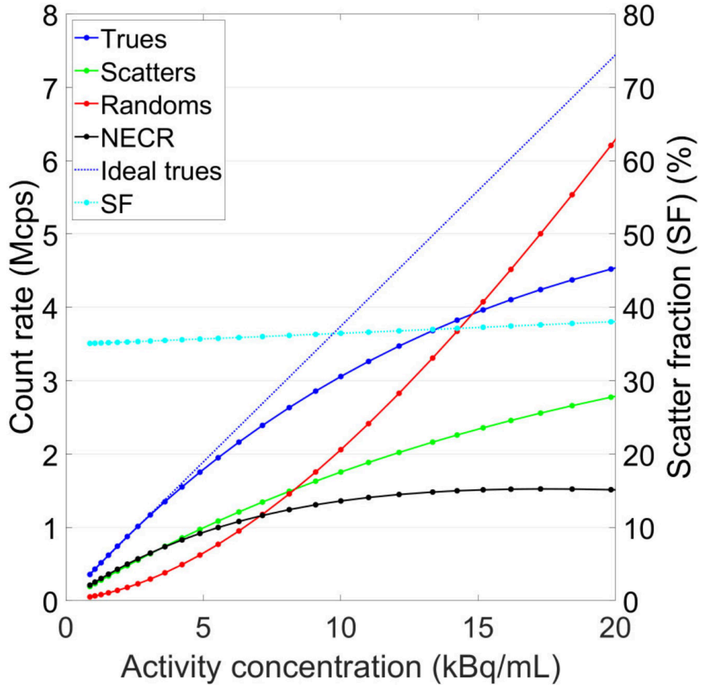
Rysunek 9.2: Measured count-rates with 70-cm-long scatter phantom. Count-rate measures are plotted vs. left vertical axes; scatter fractions are plotted vs. right vertical axes. Figure was adapted from [129].
