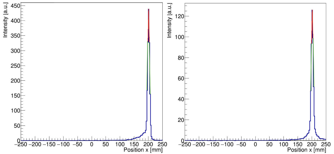
Rysunek 8.25: FWHM and its uncertainty estimation for distribution along x -axis performed at position (20,0,18.75), (left ) for TOF reconstructed image, it is equal to 7.38 \pm 0.37 \text{ mm} , and (right) Non-TOF reconstructed image, it is equal to 7.53 \pm 0.10 \text{ mm} .
