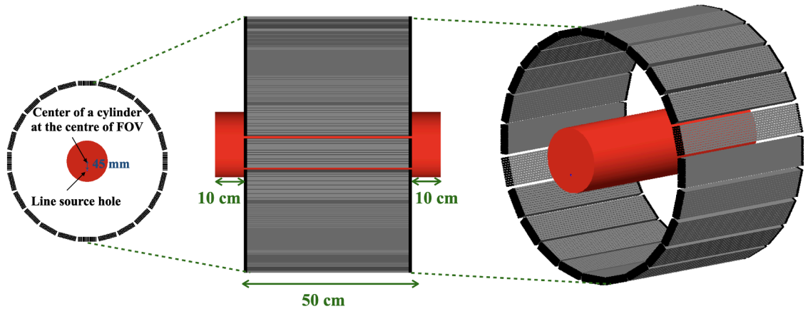
Rysunek 6.4: (Left): Cross section of 24-Module J-PET, display the place of source and phantom inside the detector, (middle): GATE visualization of side of 24-Module J-PET with NEMA scatter phantom (red color) in the center of the detector. (Right): GATE visualization of 24-Module J-PET with NEMA scatter phantom.
