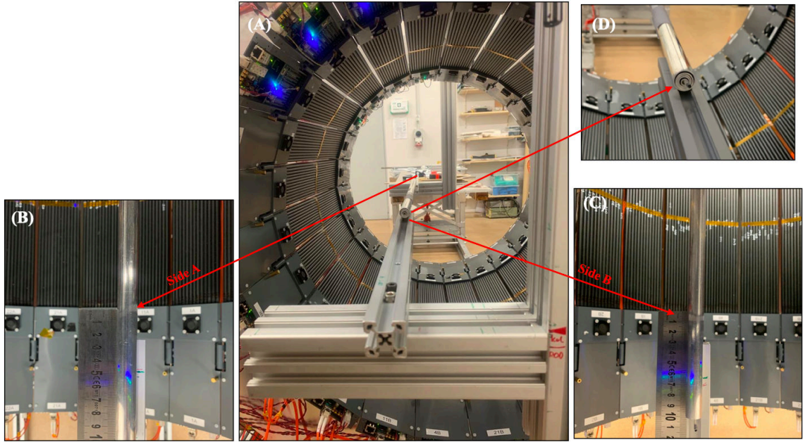
Rysunek 7.8: (A): Depicts the arrangement of the 5 sleeves of the sensitivity phantom inside the Modular J-PET, positioned at the center of the detector. (B) and (C) respectively illustrate Side A and Side B of the detector, showcasing the 10 cm extension of the sensitivity phantom beyond the AFOV. These images also highlight the strategic placement of aluminum supports on the exterior of the detector’s axial field of view. (D): Provides a zoomed-in view of the sensitivity phantom, offering a detailed depiction of all the sleeves.
