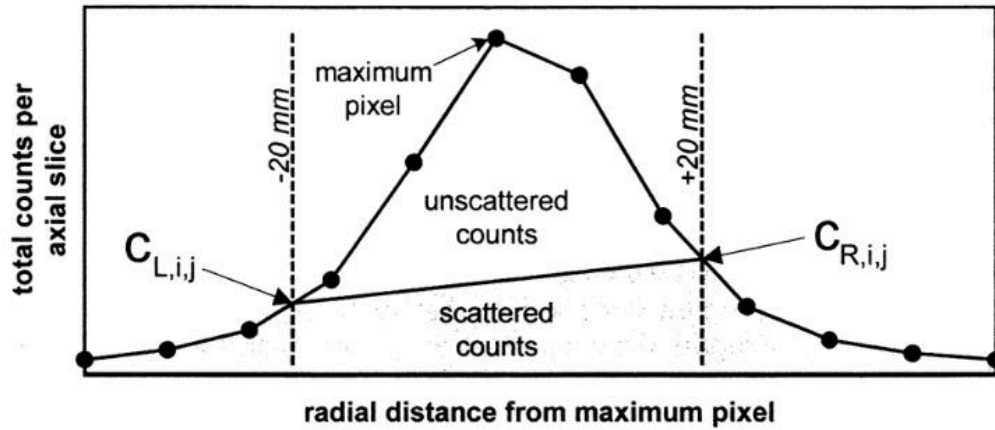
Rysunek 4.3: Integration of background counts inside and outside of 40 mm strip. Figure adapted from [6]
