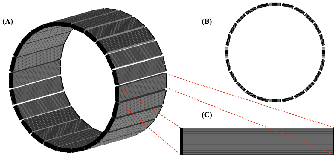
Rysunek 5.1: (A): Geometries of the Modular J-PET prototype simulated in the GATE software, (B): Cross section of 24-Module J-PET, (C): GATE visualization of one module of Modular J-PET. The plastic scintillator strips are depicted in gray, while the SiPMs on both sides of the module are displayed in black.
