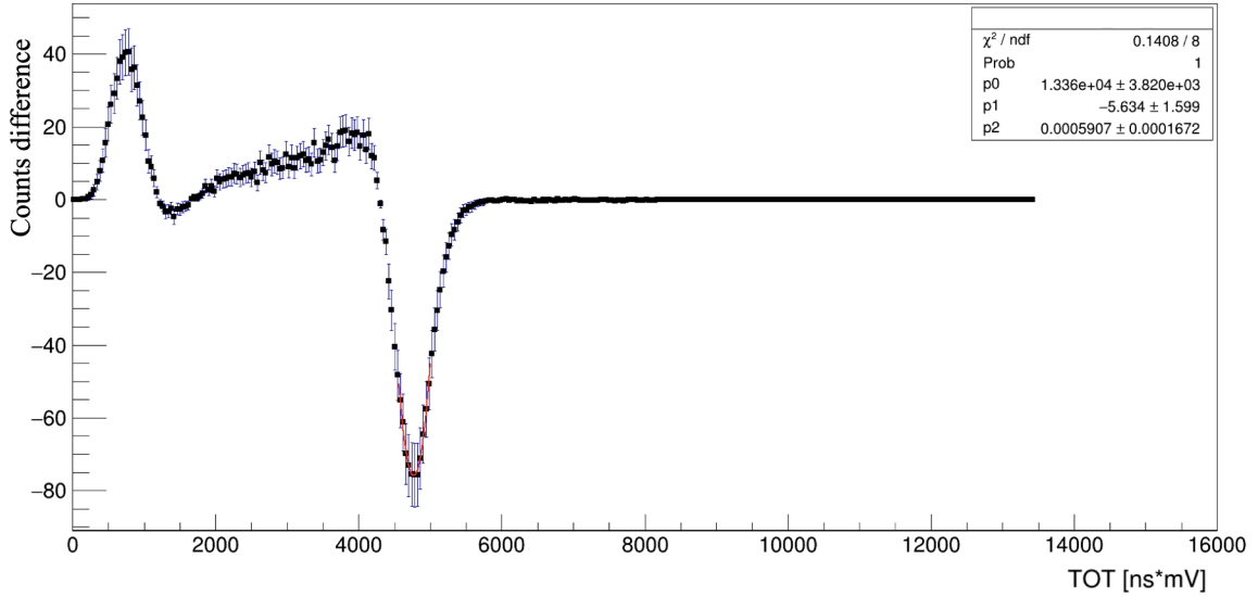
Rysunek 7.24: The first derivative of the smoothed histogram was obtained, and the associated error bars were calculated by summing the uncertainties of two consecutive points derived from the smoothed histogram.
