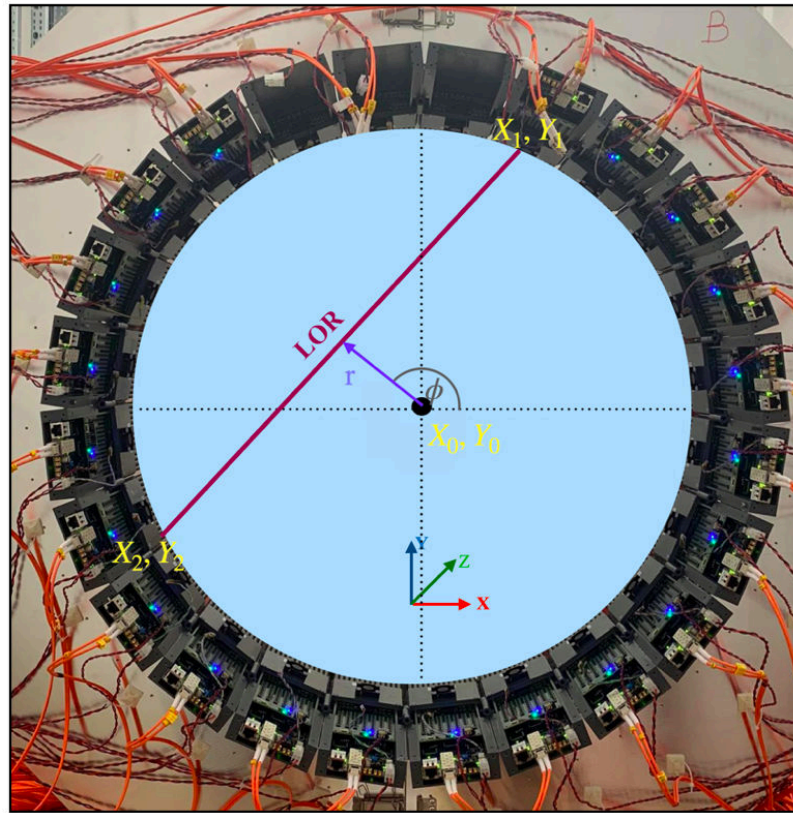
Rysunek 8.9: Illustrates the LOR represented as a line connecting two interaction points, and the subsequent conversion of the LOR into sinogram format.
