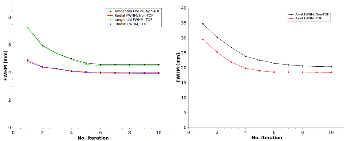
Rysunek 6.17: FWHM values as function of the iteration number for positions (1,0,0) in three directions. (left): radial and tangential FWHM with TOF and Non-TOF image reconstruction methods, (right): Axial FWHM with TOF and Non-TOF image reconstruction methods.
