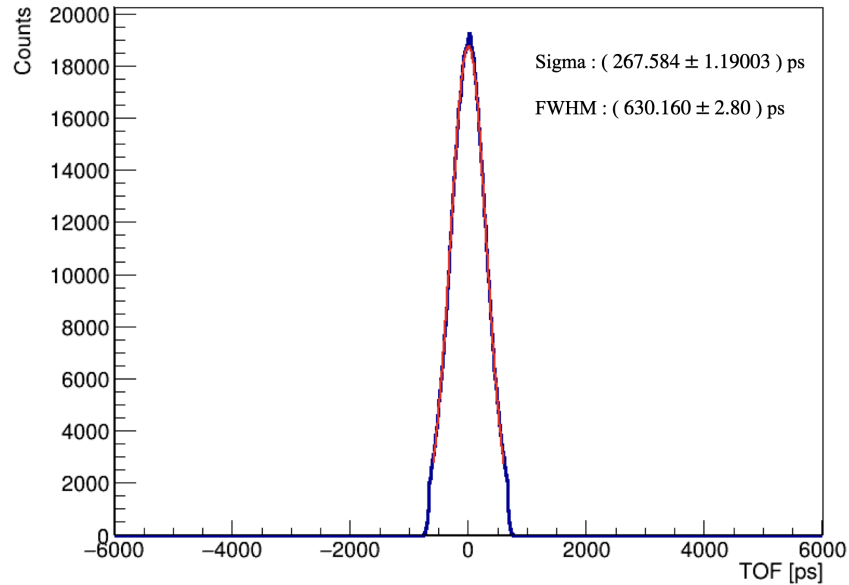
Rysunek 8.17: TOF spectrum for preselected data for Modular J-PET scanner from the 6 hours measurement with the ^{65}\text{Ge} Line source inside the 5 sleeve sensitivity phantom in the center of the FOV Modular J-PET.
