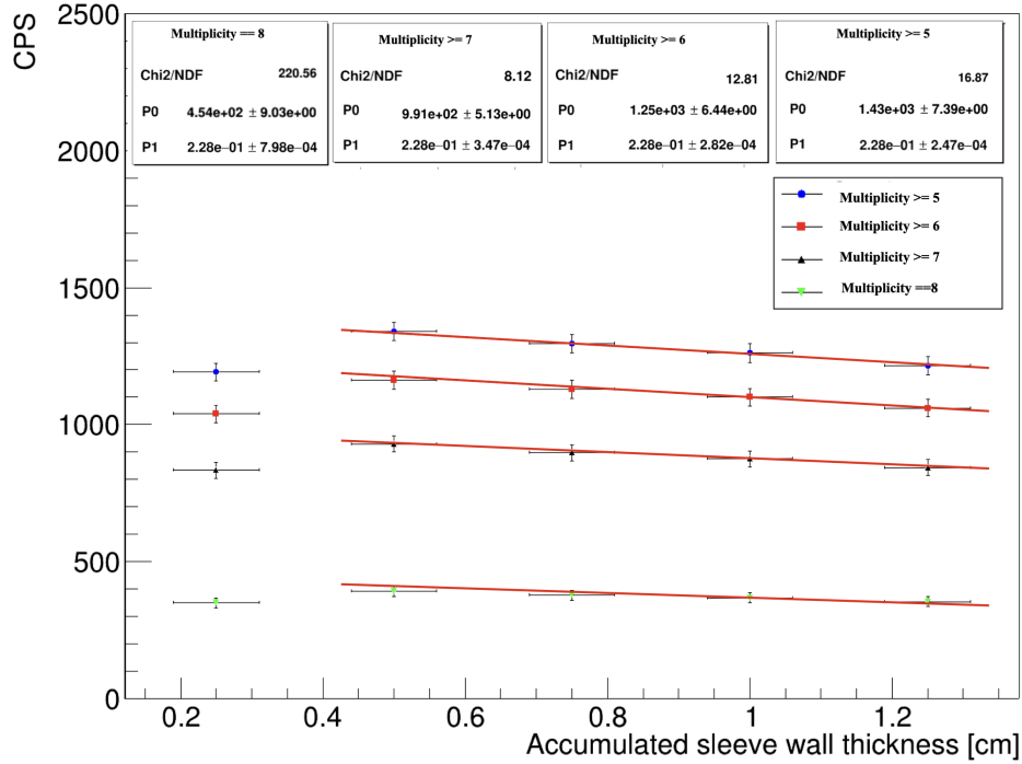
Rysunek 8.7: Illustrates R_j (Counts Per Second) as function of the accumulated sleeve wall thickness. These measurements were obtained at the center of the detector for different multiplicity cuts, and the data is fitted to the equation specified in Eq. 4.3.
