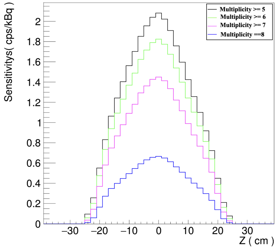
Rysunek 8.8: Axial sensitivity profile for the smallest sleeve in the center of the FOV detector for different multiplicity cuts.
