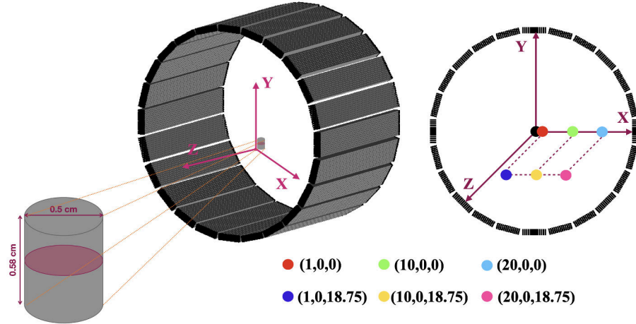
Rysunek 6.9: (Left) Representation of axis orientation in the Modular J-PET detector and exemplary of the ^{22}\text{Na} source inside the phantom in position (1, 0, 0) . ^{22}\text{Na} is in the center of aluminum phantom and active area is such as circle plane in the half of the phantom length. (Right) Schematic illustration of source positions within the Modular J-PET, black point shows the center of the detector. Please note that the figure is not drawn to scale. The unit of position measurement is in cm.
