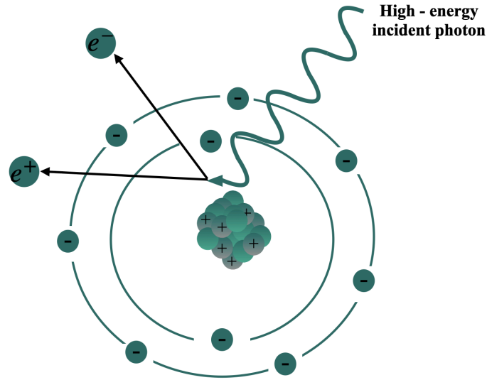
Rysunek 2.3: An illustration of electron-positron pair production, When the gamma photon energy is higher than 1.022 MeV, the photon interacts with the nucleus of an absorber atom during its passage through it and produces a positron and an electron. Figure adapted from [41].
