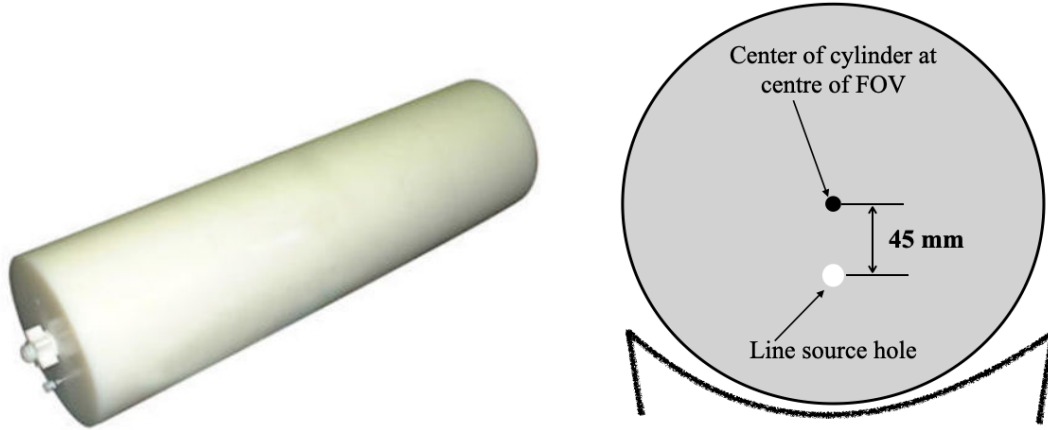
Rysunek 4.2: (Left): Scatter phantom consist of three segments which assembled together during measurements, (right) : Positioning of scatter phantom on the bed.
