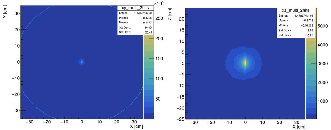
Rysunek 7.15: Control histogram of annihilation point after two hits and multiplicity selection criterion in 4 ns coincidence time window: (Left) XY position of annihilation point and, (Right) XZ position of annihilation point. It is important to note that this is from the a point like ^{22}\text{Na} source measurement, which is elongated along Z due to worse resolution of hit coordinate determination at this axis.
