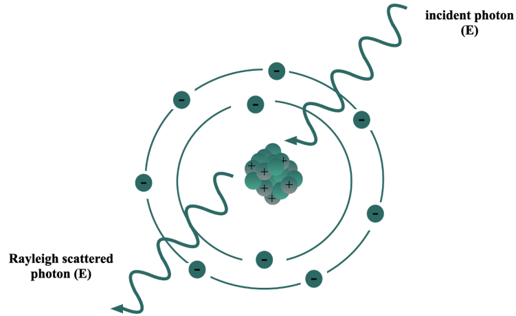
Rysunek 2.4: An illustration of Rayleigh scattering, when the gamma quantum interacts with an entire atom. Direction of scattered photon changes but its energy remains unchanged. Figure adapted from [43].
