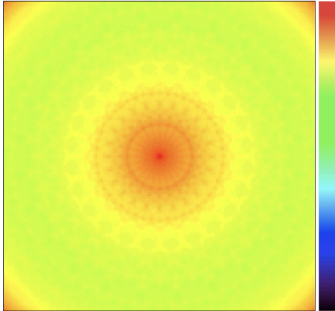
Rysunek 6.10: Transverse plane (-25 cm , 25 cm) representation extracted from the sensitivity map of the Modular J-PET, generated using QETIR software.
