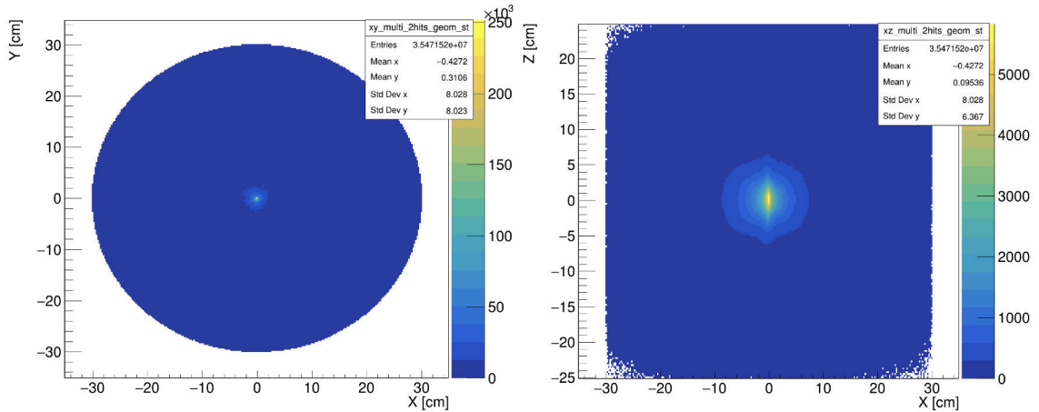
Rysunek 7.21: Control histogram of annihilation point after applying scatter test cuts to pre-selection criteria in 4 ns coincidence time window: (Left) XY position of annihilation point and, (Right) XZ position of annihilation point. It is important to note that this is from the a point like ^{22}\text{Na} source measurement, which is elongated along Z due to worse resolution of hit coordinate determination at this axis.
