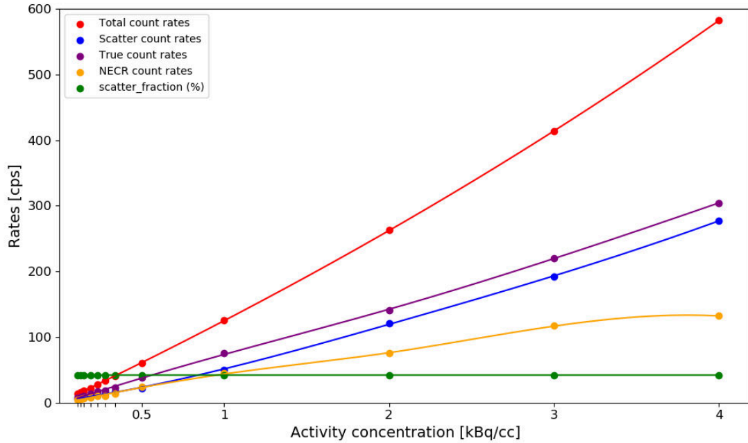
Rysunek 6.8: Count rates of different types of coincidences and NECR as a function of activity concentration (in kBq/cc).
