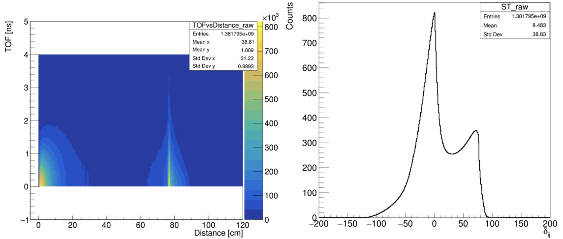
Rysunek 7.19: (Left): Two-dimensional histogram depicting the spatial separation as a function of Time of Flight (TOF) for all events, (Right): Illustrates \delta_{i,j} = d_{i,j} - c \times \Delta t_{i,j} . Secondary scattering interactions are identifiable by small \delta_{i,j} values and are subsequently excluded from consideration. Interactions with \delta_{i,j} more than 40 cm are designated as primary photon candidates.
