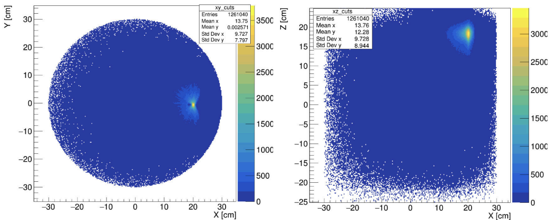
Rysunek 8.16: Histogram of annihilation points for position (20,0,18.75): (Left) XY projection of annihilation point and, (Right) XZ projection of annihilation points.
