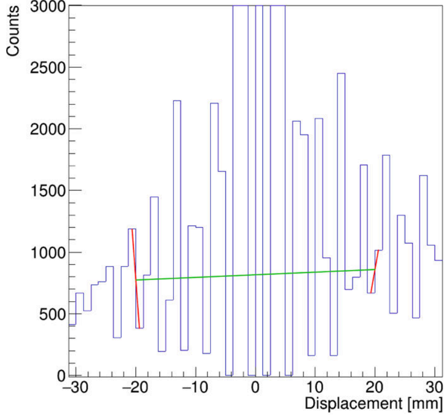
Rysunek 8.13: Graphical explanation of determination of linear interpolation between middle point of two nearest bins at \pm 20 mm, which a_{left} , b_{left} , a_{right} , and b_{right} is equal to -643.08, -12076.5, 278.667, and -4731.96, respectively.
