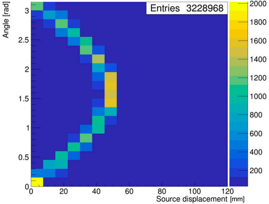
Rysunek 8.11: Depicts the final sinogram, which was reprocessed within the ROOT environment for visual clarity. Notably, this particular sinogram was excluded from subsequent analyses.
