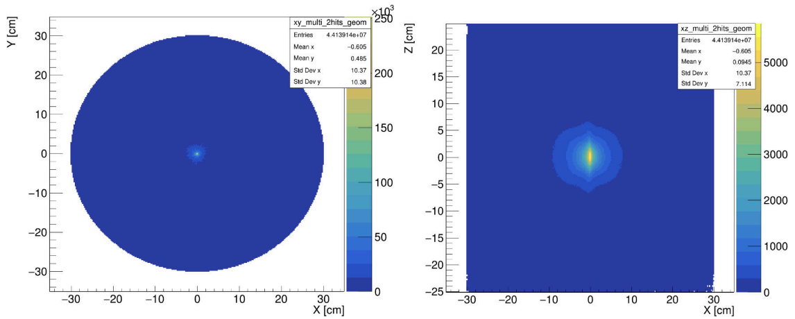
Rysunek 7.18: Control histogram of annihilation point after applying geometry cuts to pre-selection criteria in 4 ns coincidence time window: (Left) XY position of annihilation point. (Right) XZ position of annihilation point. It is important to note that this is from the a point like ^{22}\text{Na} source measurement, which is elongated along Z due to worse resolution of hit coordinate determination at this axis.
