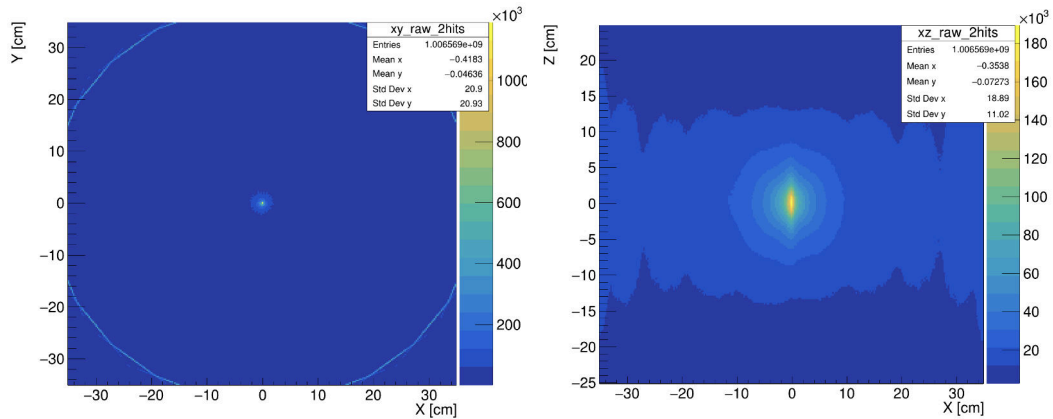
Rysunek 7.13: Control histogram of annihilation point after two hits selection criterion in 4 ns coincidence time window: (Left) XY position of annihilation point and, (Right) XZ position of annihilation point. It is important to note that this is from the a point like ^{22}\text{Na} source measurement, which is elongated along Z due to worse resolution of hit coordinate determination at this axis.
