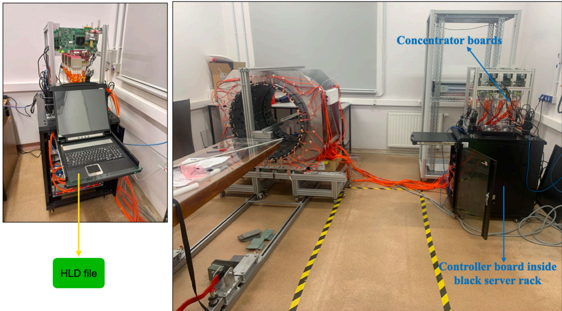
Rysunek 3.5: (Right): Display the placement of the Modular J-PET, patient bed, data acquisition system (DAQ) Modular J-PET. (Left): The DAQ is the integration of several components which consists of sensors, DAQ measurement hardware, the output/display module, and a computer with programmable software. It also contains the control module that store the digital data of the Modular J-PET detector [87].
