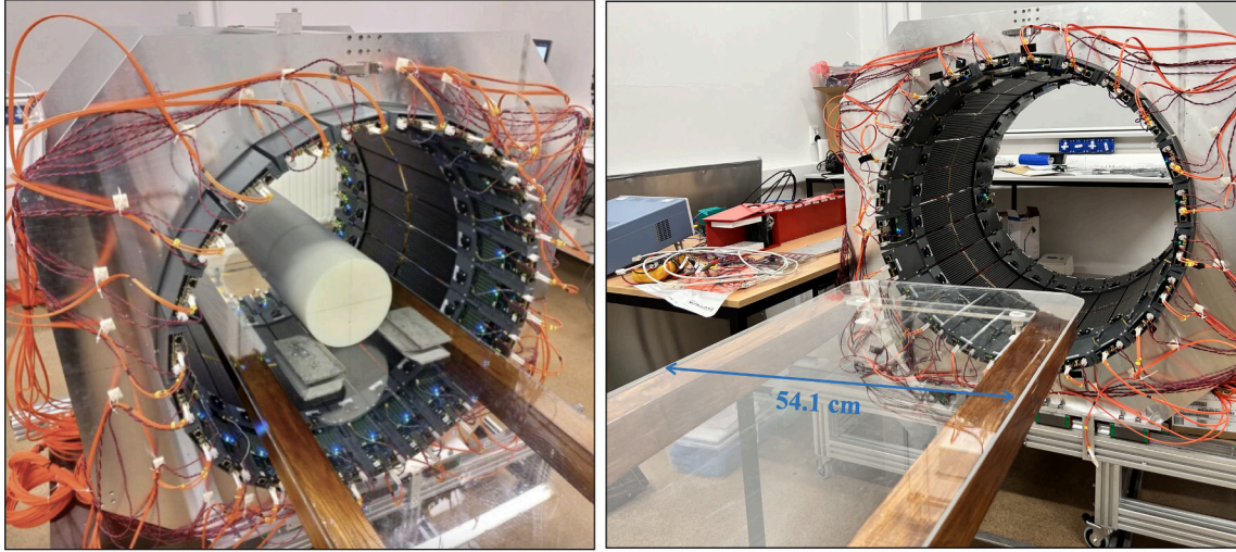
Rysunek 7.10: (Right): Depicts the experimental setup for scatter fraction measurement. the bed including the plexi and wooden. (left): Displays the PET scatter phantom placed on the dedicated bed.
